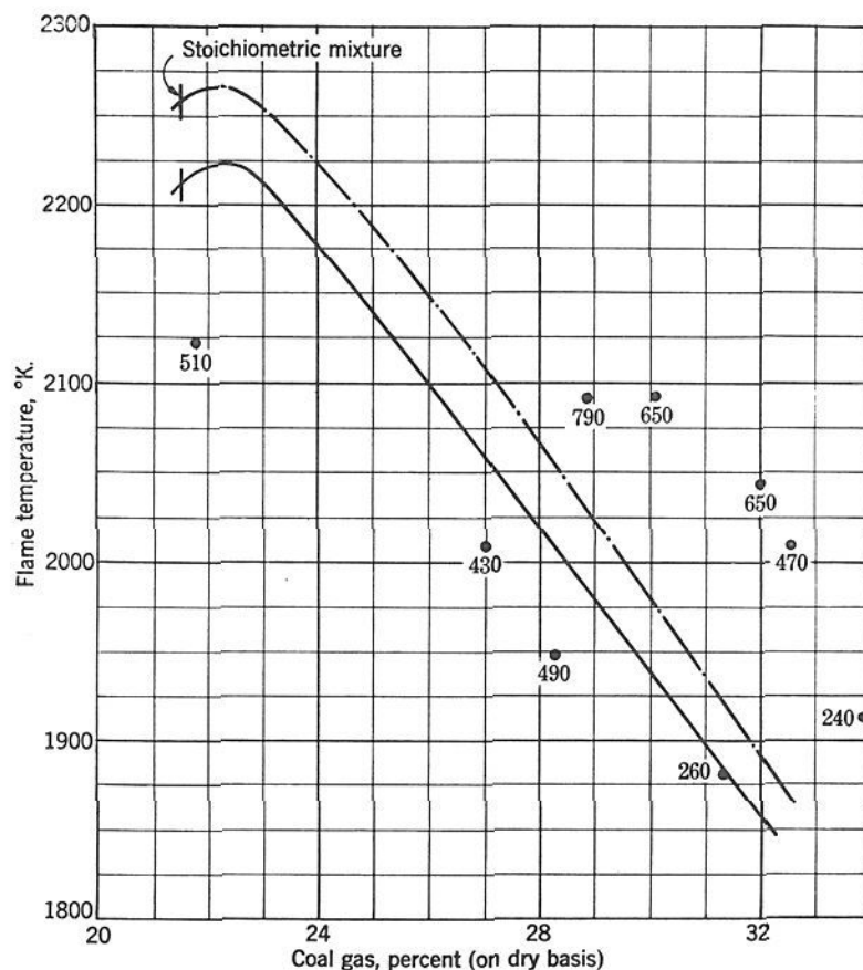
FIG. 1. Comparison of theoretical flame temperatures of coal gas-air mixtures with experimental flame temperatures determined by the line-reversal method. — · —, theoretical curve, dry mixtures; ———, theoretical curve, moist mixtures; ●, sodium line-reversal flame temperatures with gas velocity in centimeters per second.
